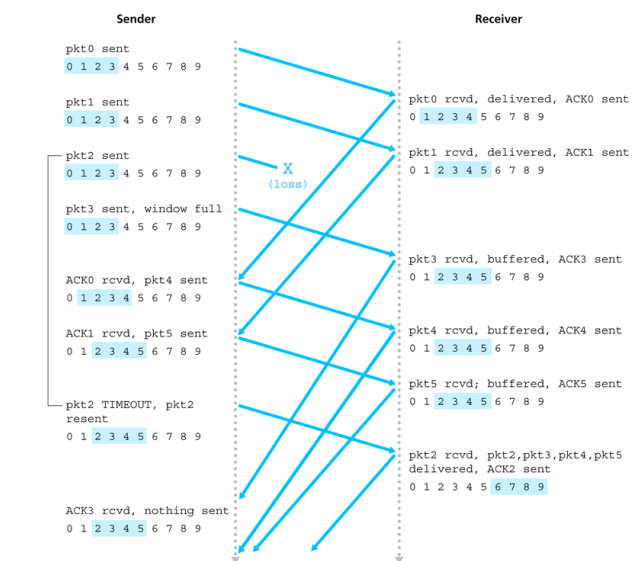
Figure 3.26 ♦ SR operation
